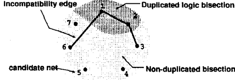
Figure 5: Incompatibility graph.
