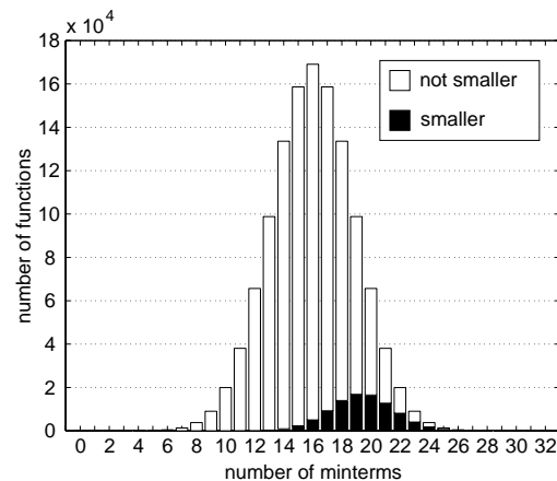
Figure 9. Heuristic method
