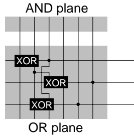
Figure 7. Product term sharing
