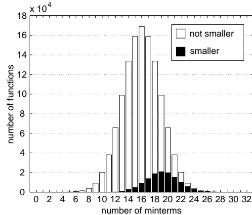
Figure 8. Exact method
