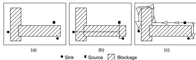
Figure 1. An example of wire buffering with placement blockages
