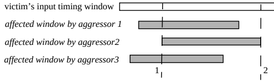
Figure 4. Sweeping affected windows
